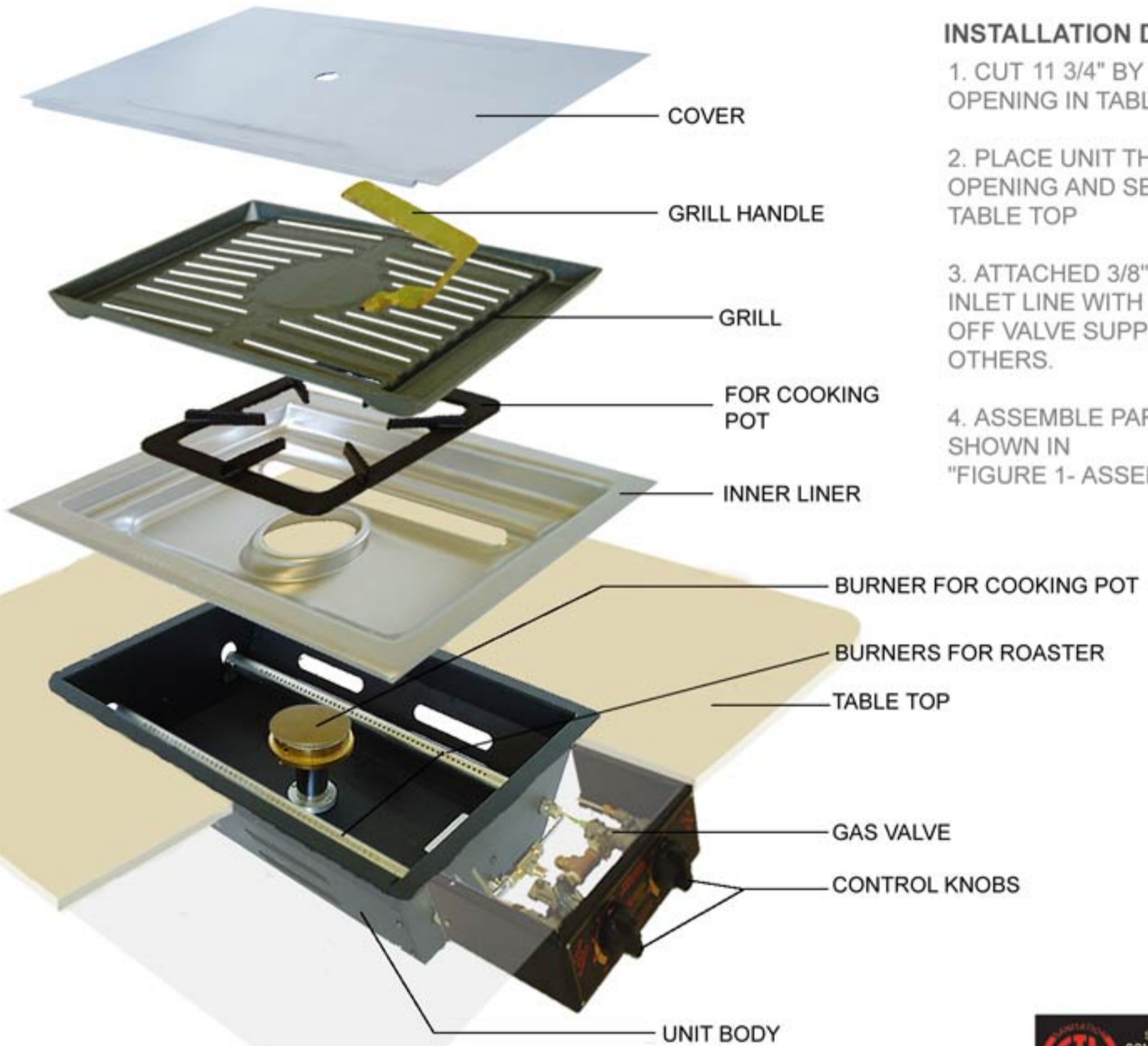
FIGURE 1 - ASSEMBLY
